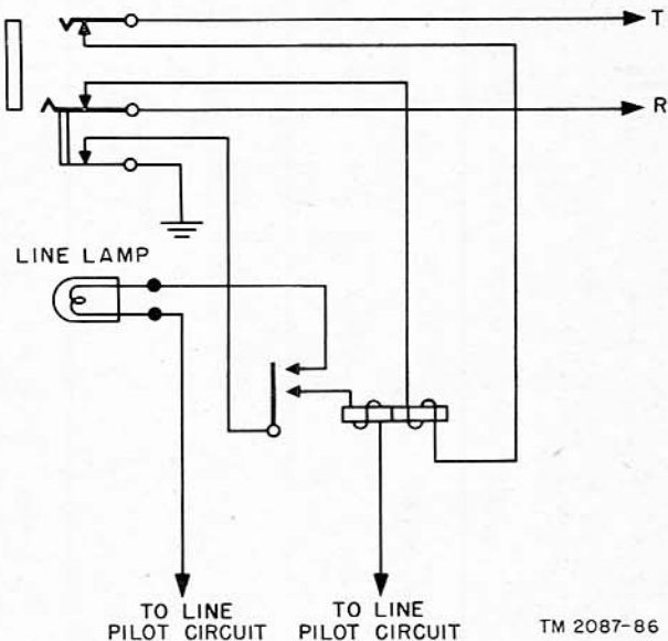
Figure 78. Universal line circuit connected for magneto operation, schematic.
