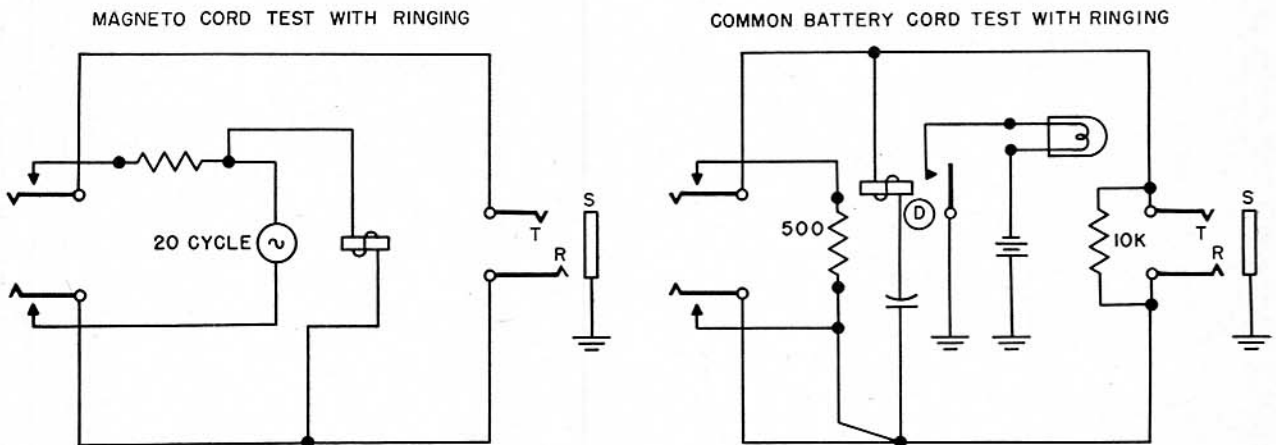
Figure 85. Cord test circuit, schematic.
