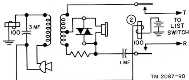
Figure 82. Operator's telephone circuit, schematic.
