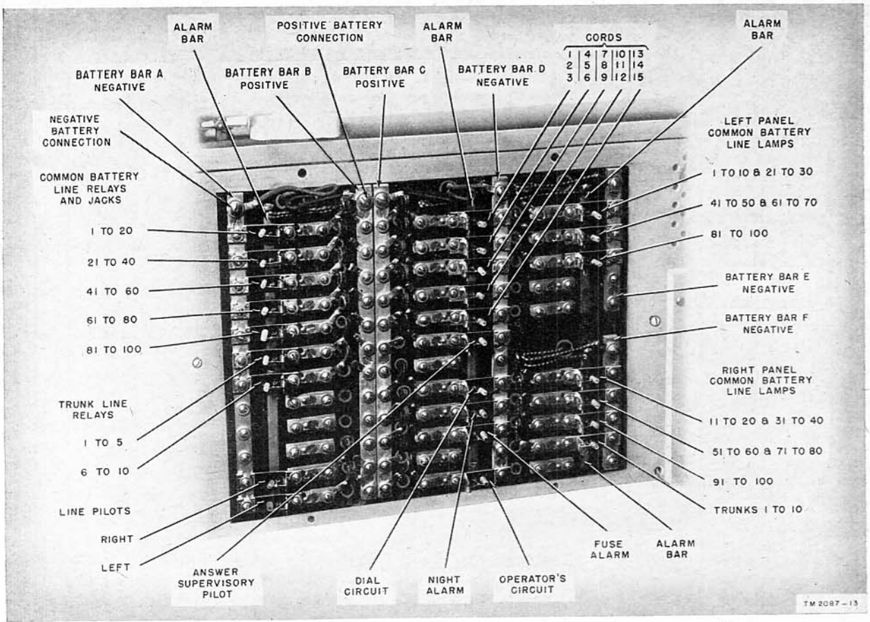
Figure 9. Switchboard SB-53 ( )/FTC (Kellogg type), fusing and power connections.
