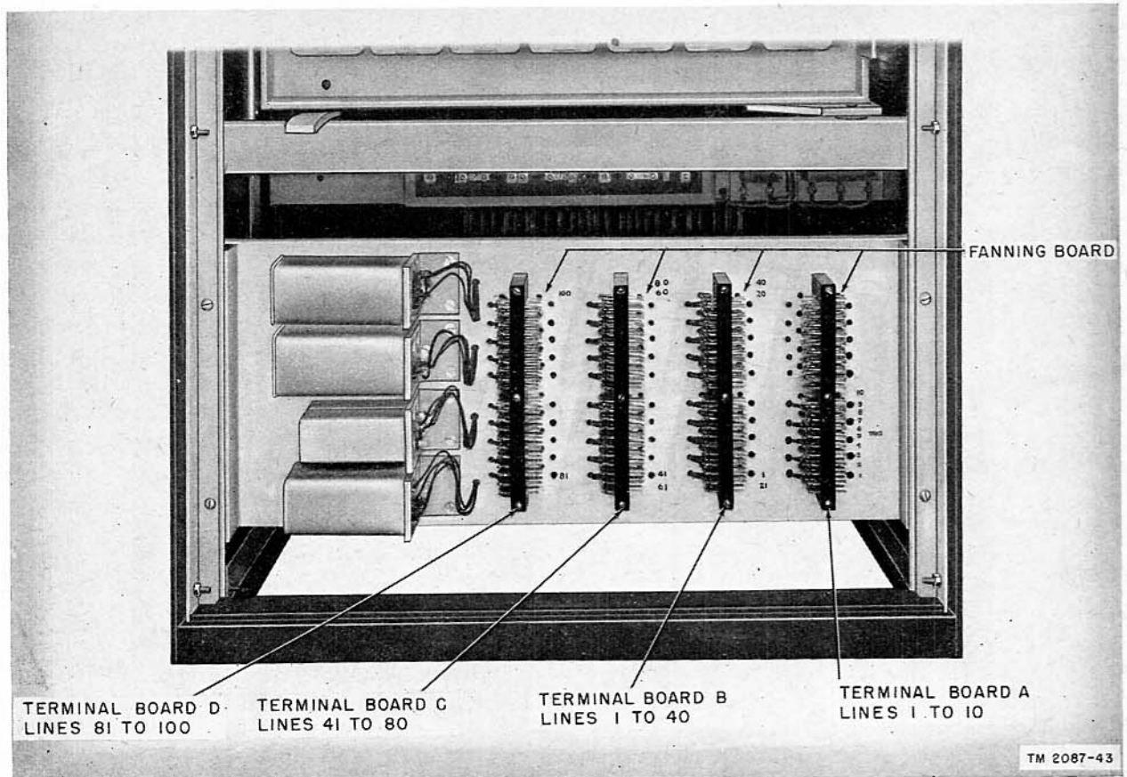
Figure 7. Switchboard SB-53 ( )/FTC (Kellogg type), fanning and terminal boards.
