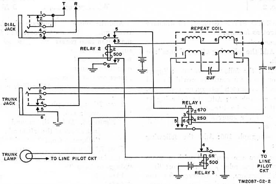
Figure 79.1. (Superseded) Switchboard SB-53A/FTC, universal trunk circuit, schematic.
