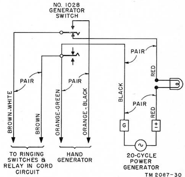
Figure 19. Generator circuit, schematic.
