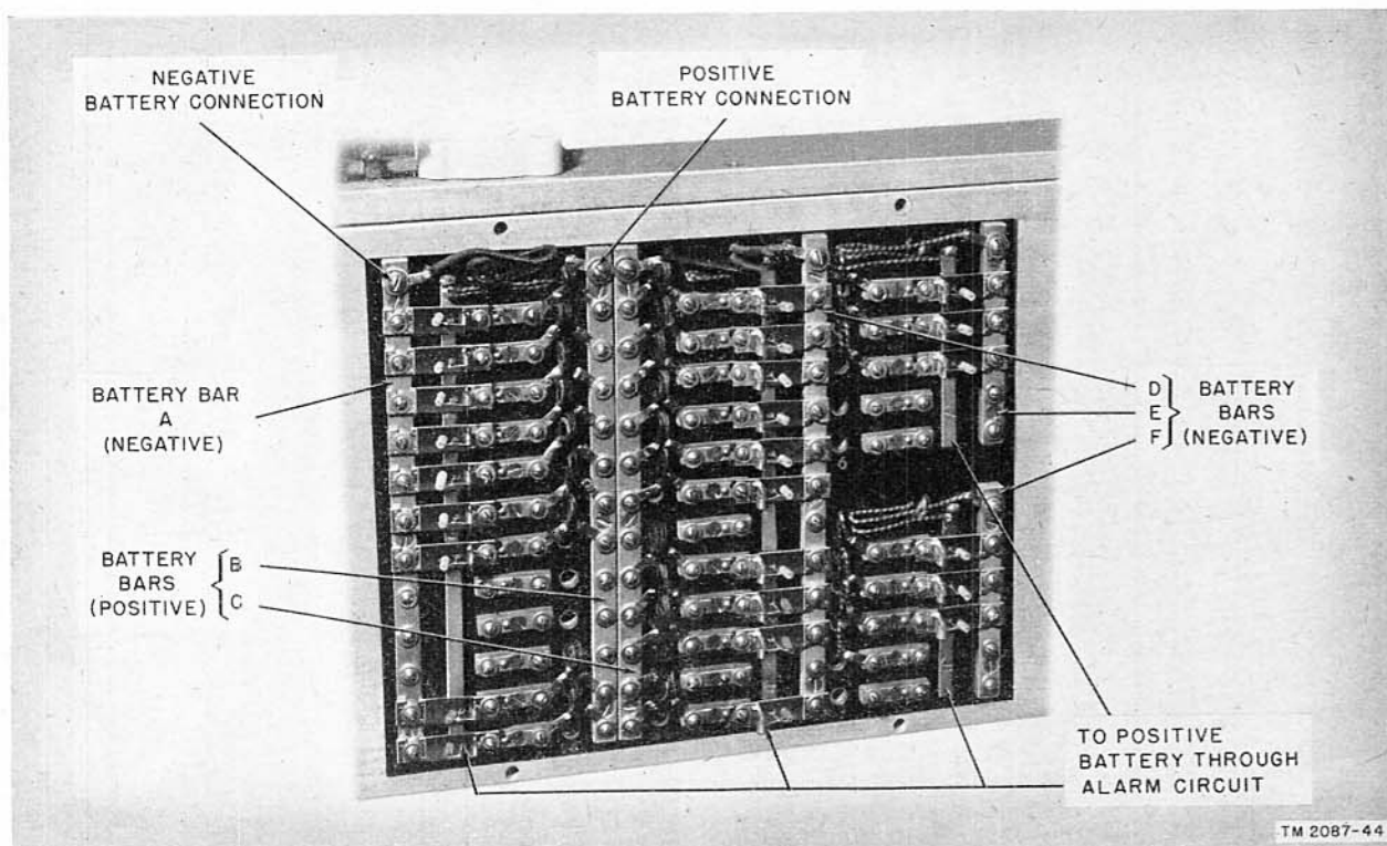
Figure 36. Battery terminals.
