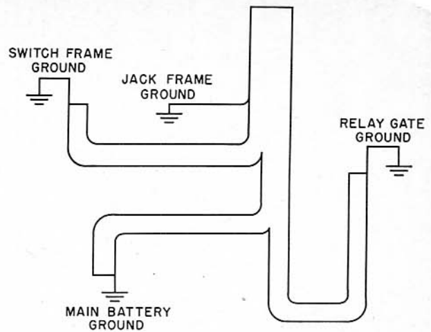
Figure 90. Ground circuit, schematic.
