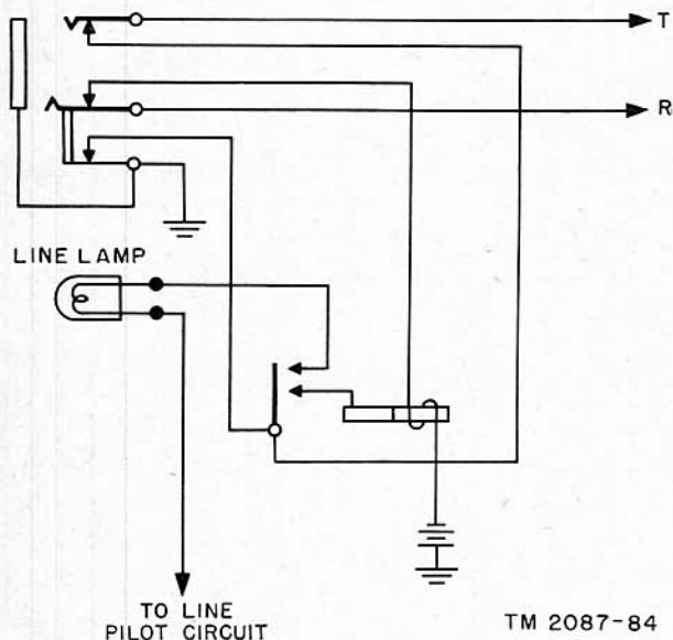
Figure 77. Universal line circuit connected for common battery operation, schematic.
