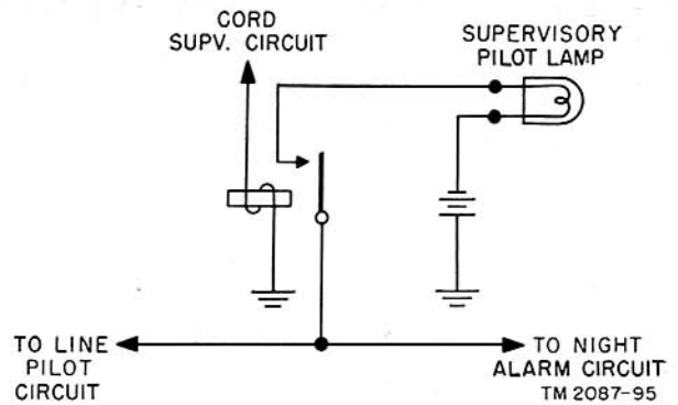
Figure 87. Supervisory pilot circuit, schematic.
