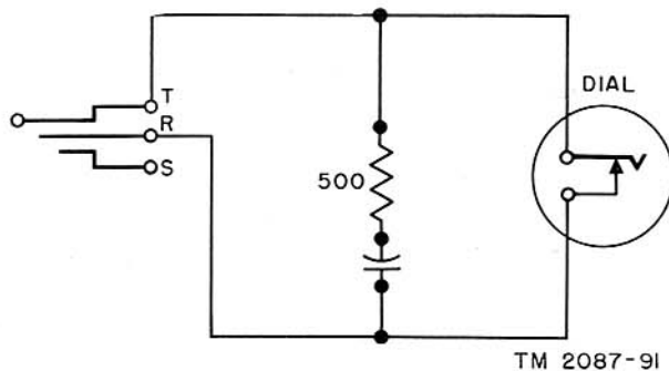
Figure 83. Dial and dial cord circuit, schematic.
