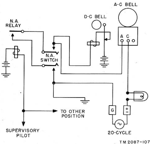
Figure 23. Night alarm circuit, schematic.
