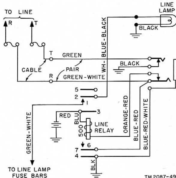
Figure 41. Universal line circuit, showing connection for common battery operation, wiring diagram
