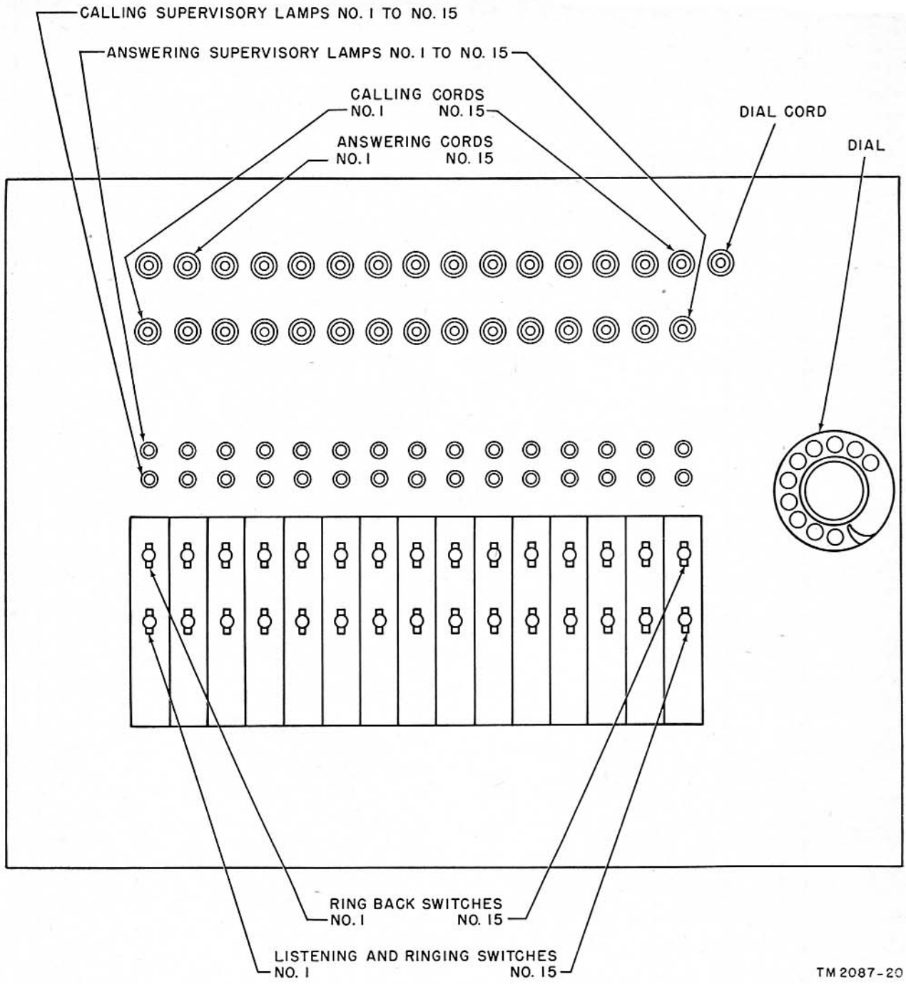
Figure 75. Switchboard SB-53( )/FTC, (Stromberg-Carlson universal type 106), top view of switch shelf, showing arrangement of cords, lamps, and switches.
