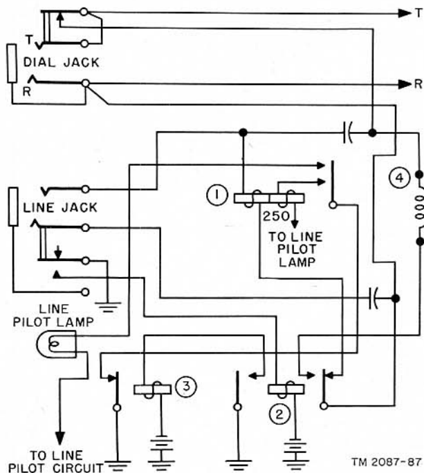
Figure 79. Universal trunk circuit connected for common battery operation, schematic.
