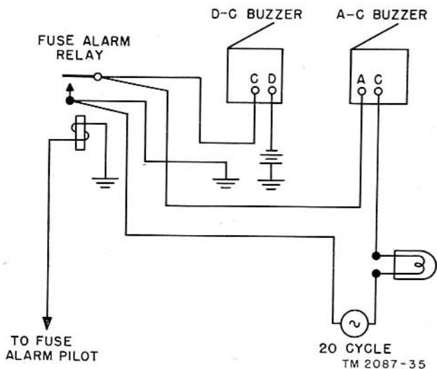
Figure 25. Fuse alarm circuit, schematic.
