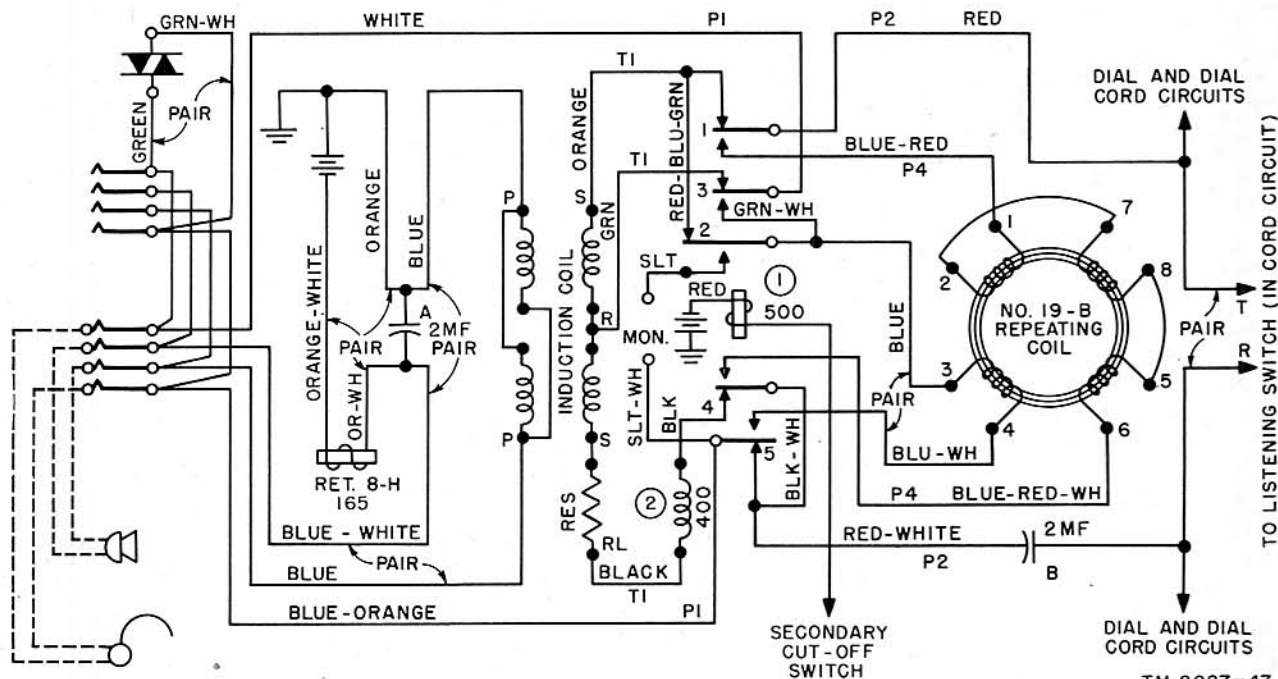
Figure 39. Operator's circuit, wiring diagram.
