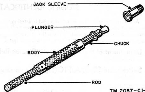
Figure 111 (Added) Switchboard SB-53A/FTC, jack sleeve tool.
