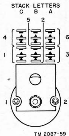
Figure 51. Spring pile-up identification diagram for Kellogg relays, terminal end view.
