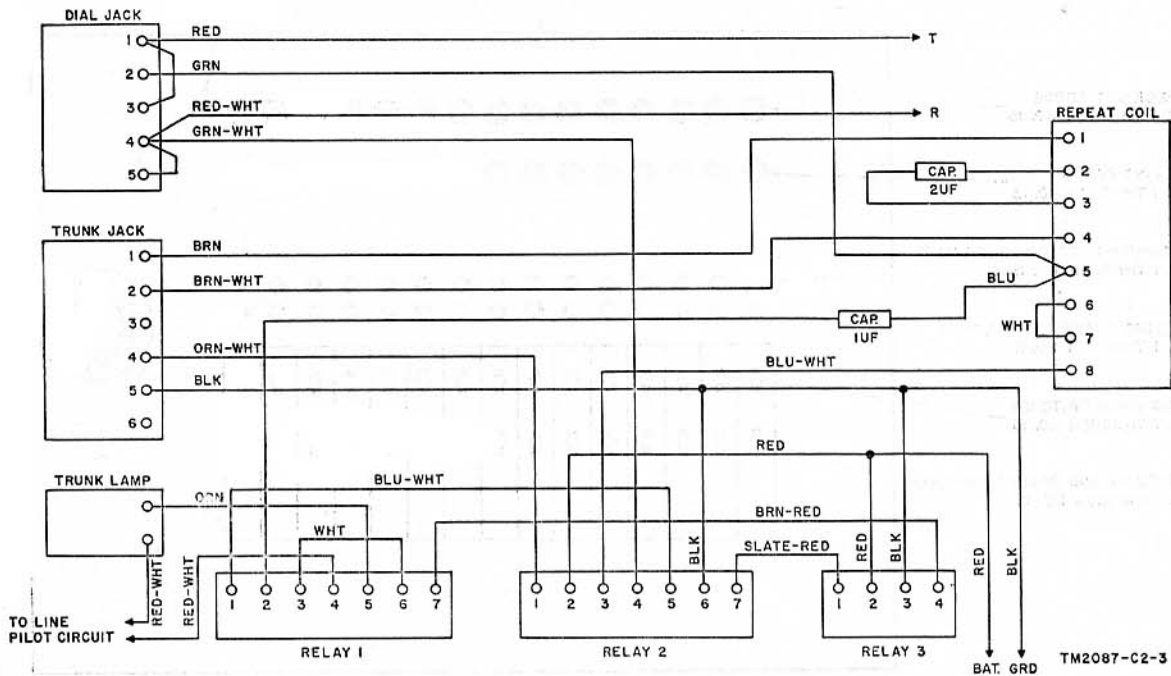
Figure 97.1. (Added) SB-53A/FTC universal trunk circuit, wiring diagram.
