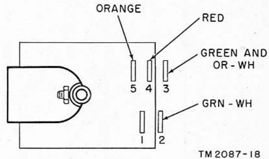
Figure 74. Switchboard SB-53( )/FTC (Stromberg-Carlson universal type 106), short lines relay wiring diagram.
