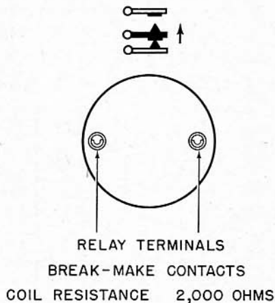
Figure 65. Winding and spring terminal arrangement of Kellogg 2102-S-HG pilot alarm relay, terminal end view.
