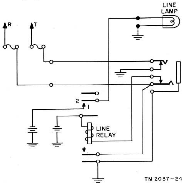
Figure 13. Universal line circuit connected for common battery operation, schematic.
