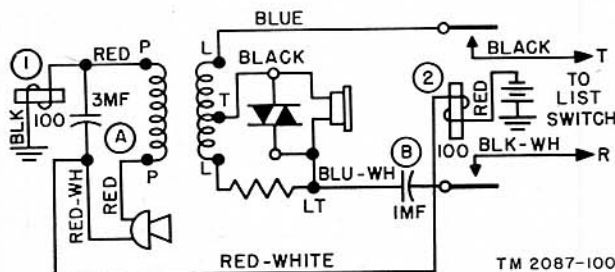
Figure 92. Operator's telephone circuit, wiring diagram.
