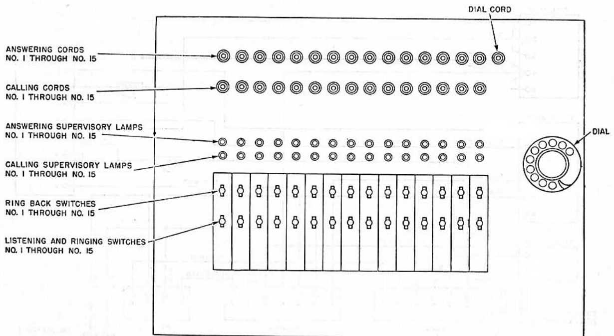
Figure 75 (Superseded) Top view of switch shelf, showing arrangement of cords, lamps, and switches.
