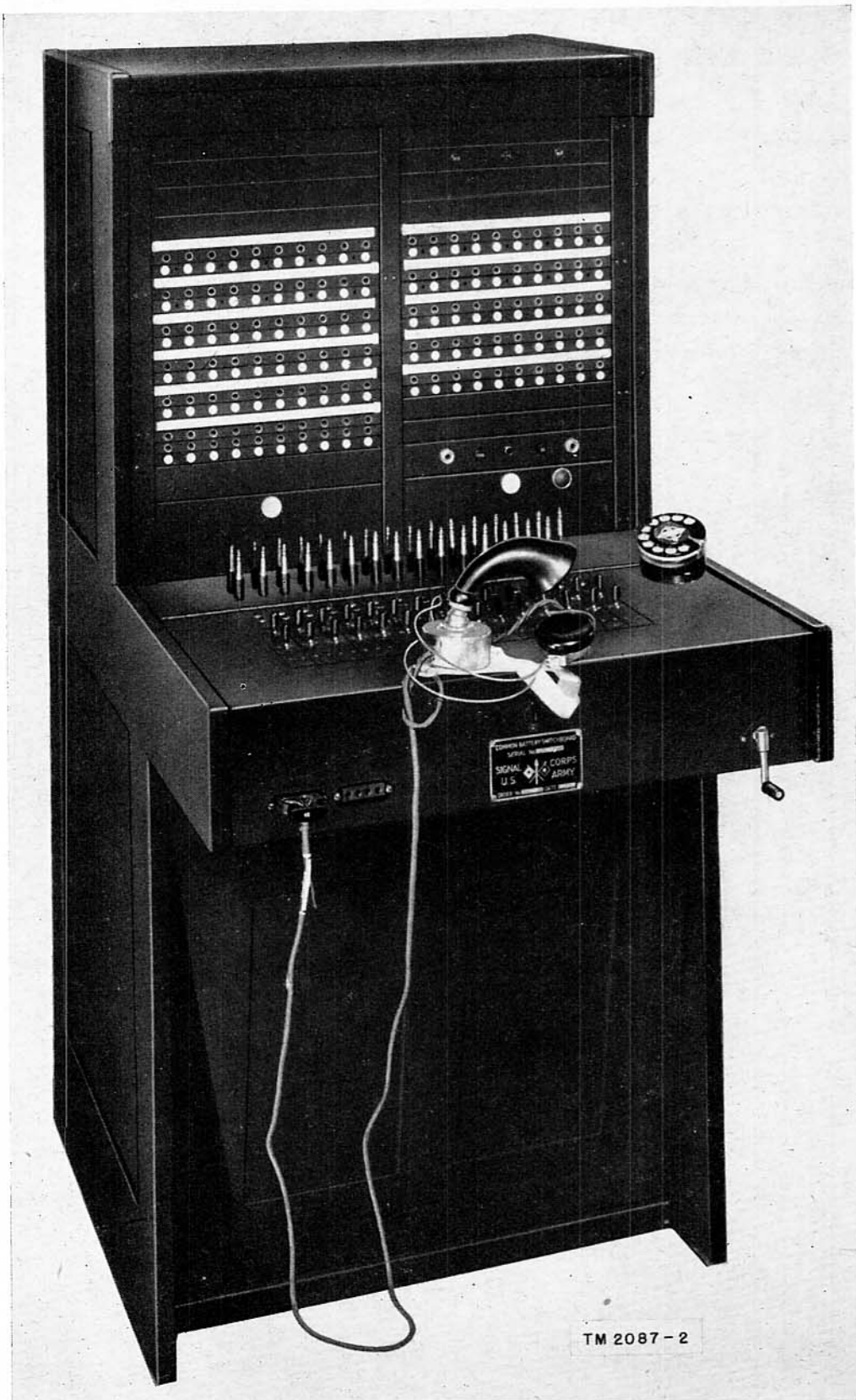
Figure 67. Switchboard SB-53( )/FTC (Stromberg-Carlson universal type 106).
