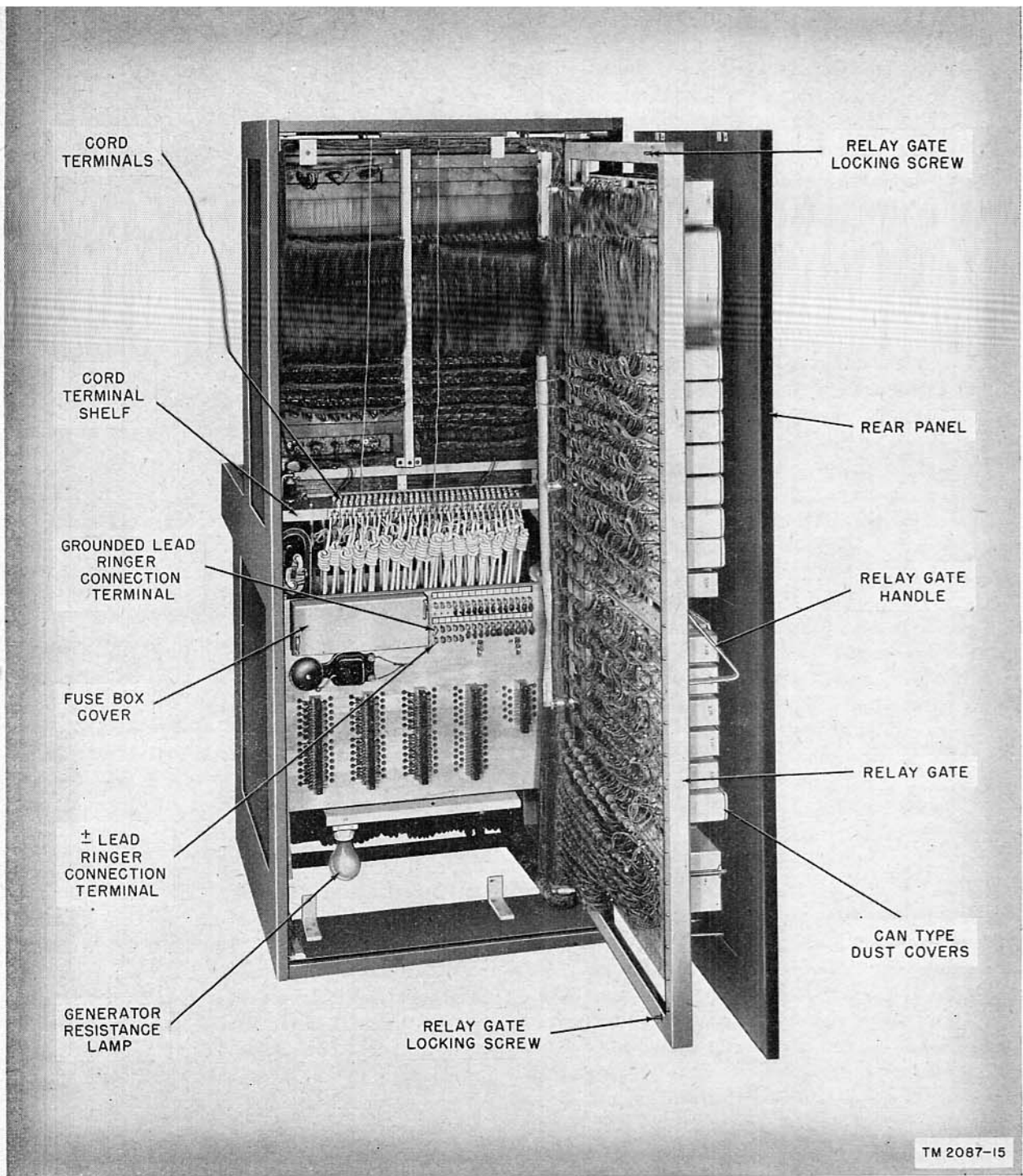
Figure 69. Switchboard SB-53( )/FTC (Stromberg-Carlson universal type 106), rear view.
