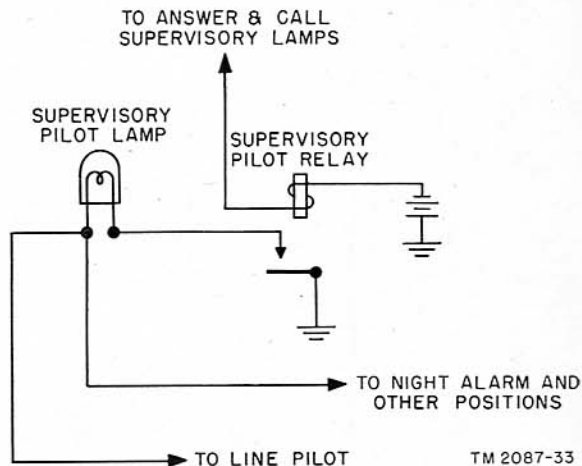
Figure 22. Supervisory pilot circuit, schematic.
