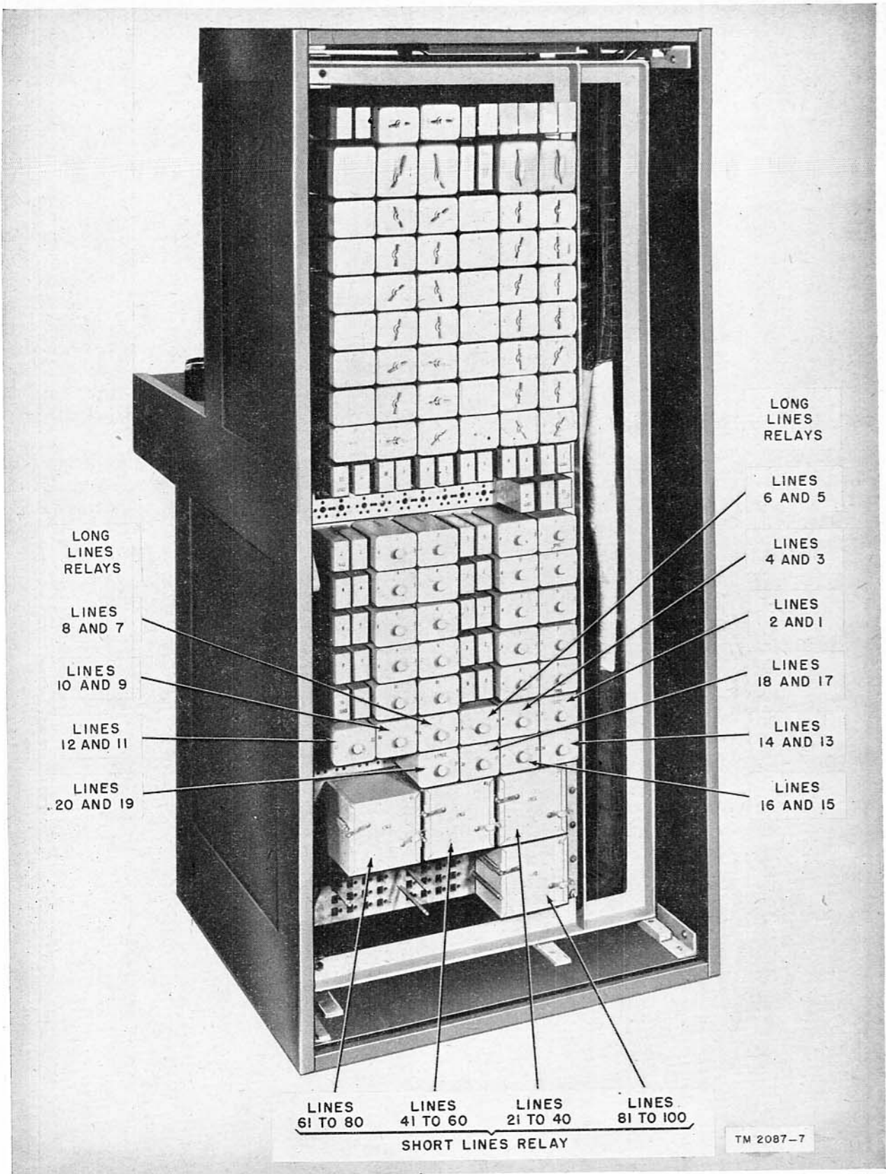
Figure 72. Switchboard SB-53( )/FTC (Stromberg-Carlson universal type 106) showing locations of long and short lines relays.
