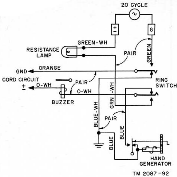
Figure 84. Generator circuit, schematic.
