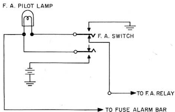
Figure 24. Fuse pilot circuit, schematic.
