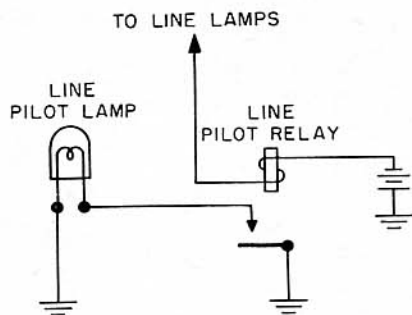
Figure 21. Line pilot circuit, schematic.
