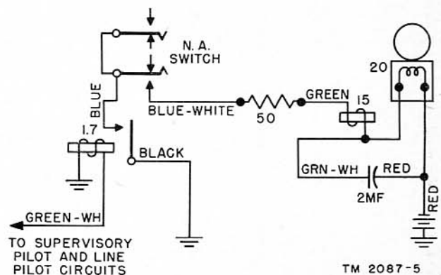
Figure 99. Night alarm circuit, wiring diagram.
