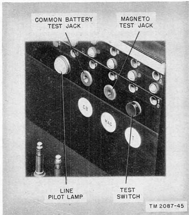
Figure 37. Cord test jacks and switch.
