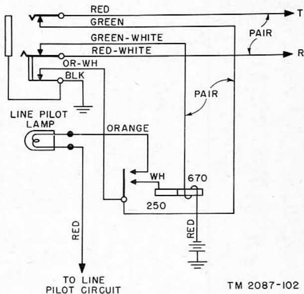
Figure 94. Universal line circuit connected for common battery operation, wiring diagram.
