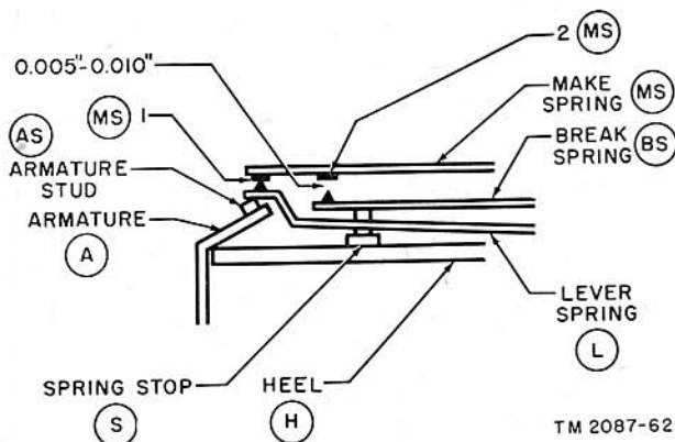
Figure 54. Make-before-break combination, operated position.
