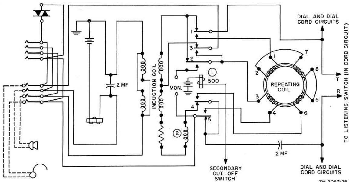
Figure 17. Operator's telephone circuit, schematic.
