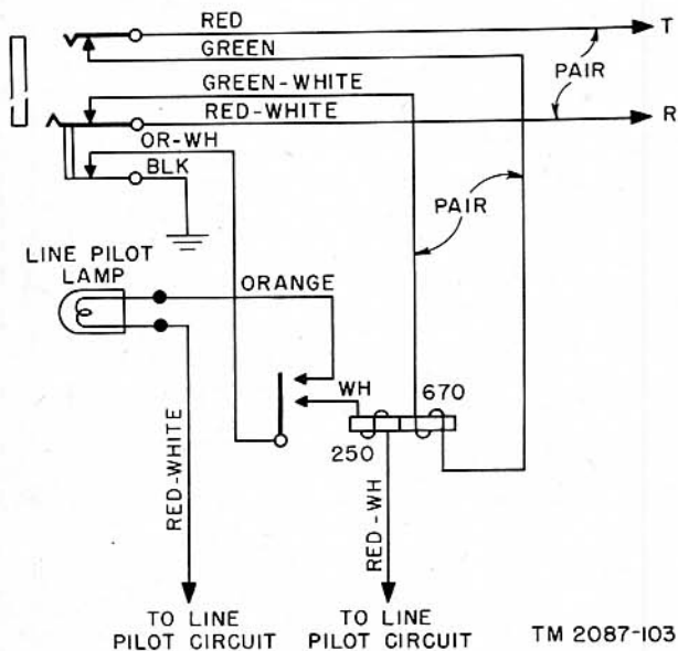
Figure 95. Universal line circuit connected for magneto operation, wiring diagram.
