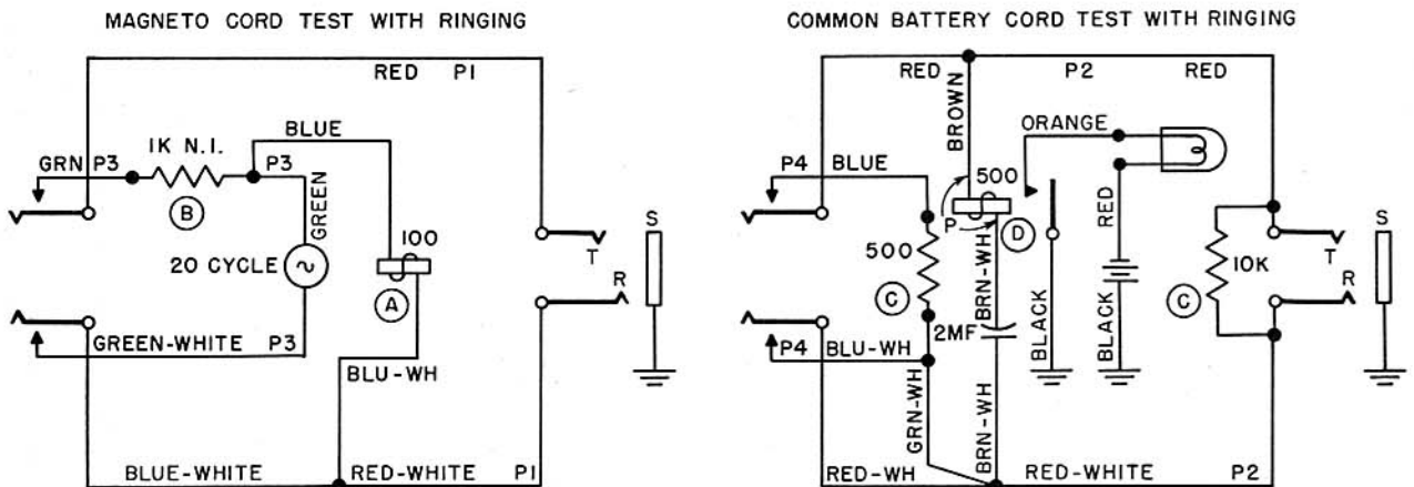
Figure 91. Cord test circuit, wiring diagram.
