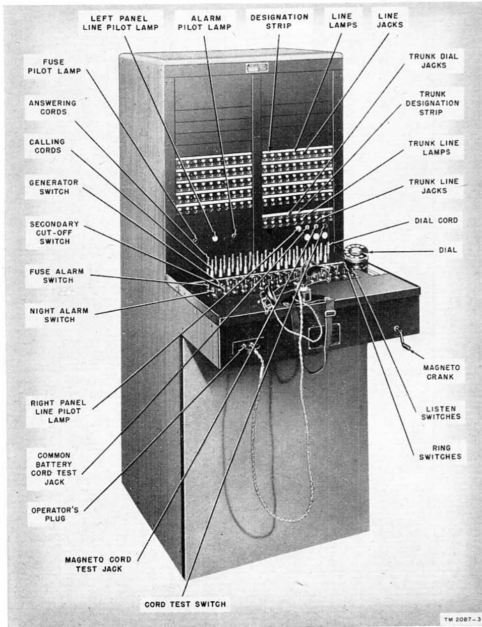
Figure 2. Switchboard SB-53 ( )/FTC (Kellogg type), front view.
