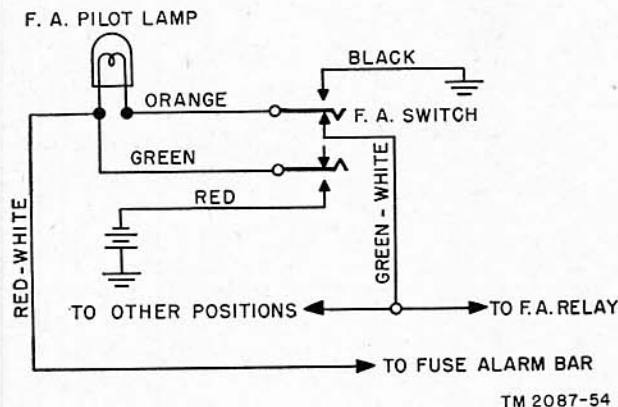
Figure 46. Fuse alarm pilot circuit, wiring diagram.
