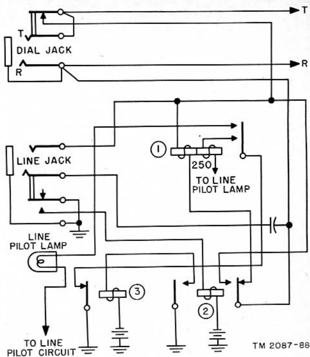
Figure 80. Universal trunk circuit connected for magneto operation, schematic.
