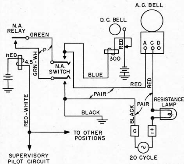
Figure 45. Night alarm circuit, wiring diagram.
