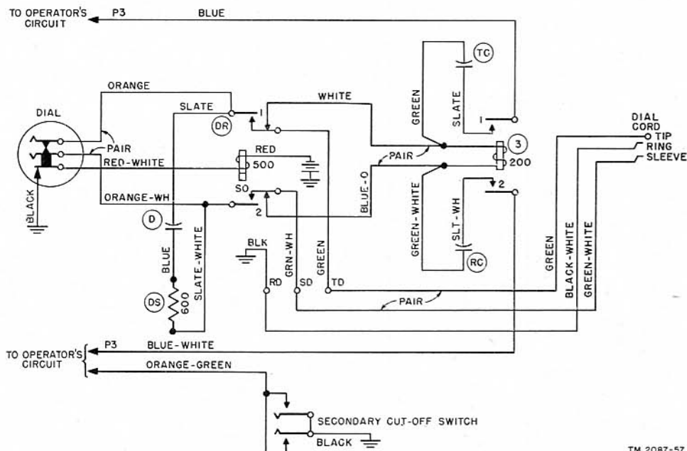
Figure 49. Dial and dial cord circuit, wiring diagram.
