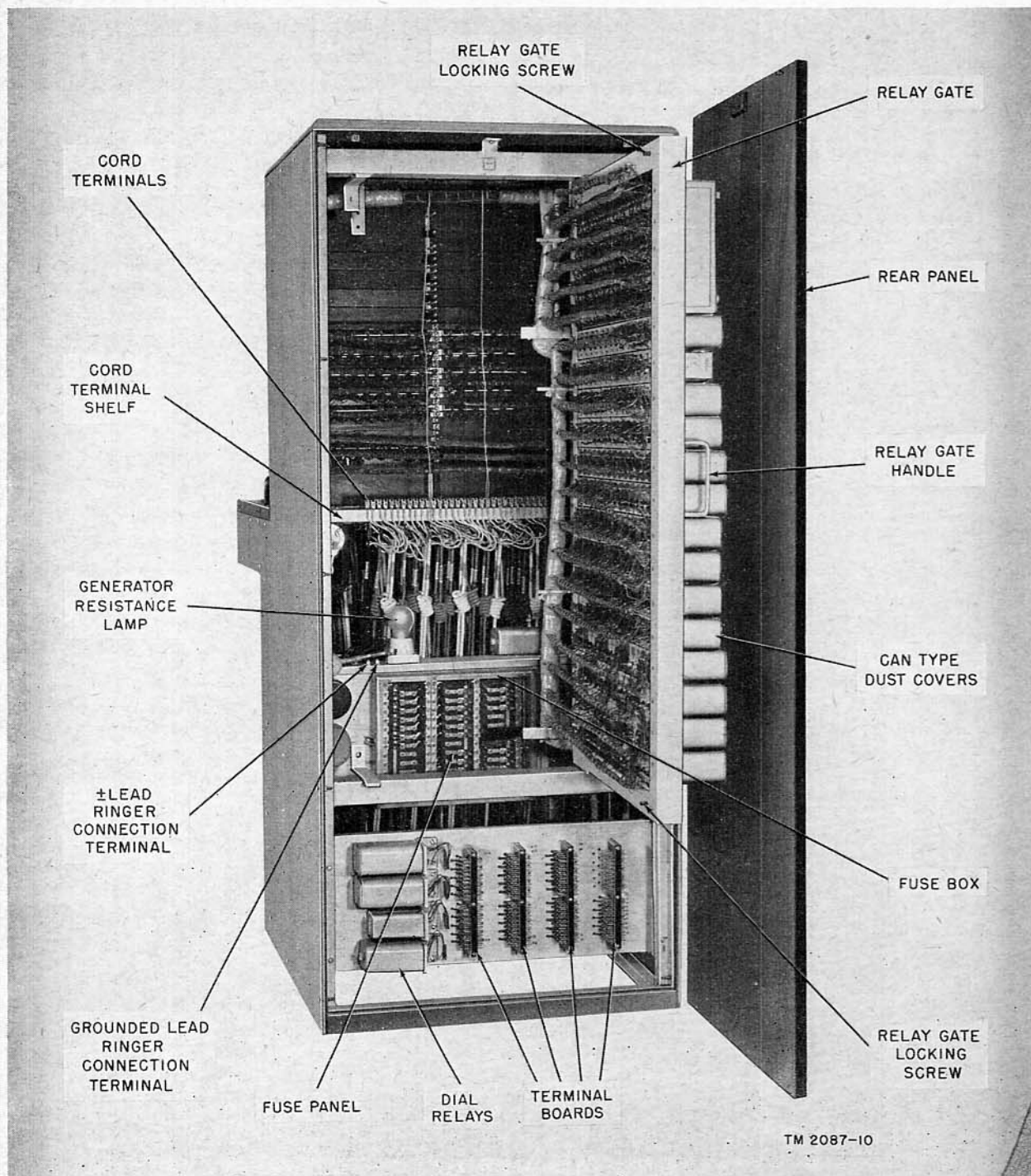
Figure 6. Switchboard SB-53( )/FTC (Kellogg type), relay gate open.
