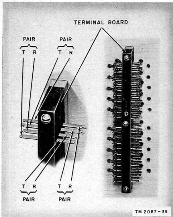
Figure 8. Switchboard SB-53( )/FTC (Kellogg type) terminal board, showing tip and ring connections.
