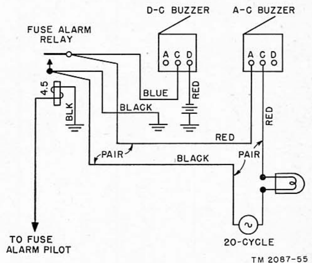
Figure 47. Fuse alarm circuit, wiring diagram.
