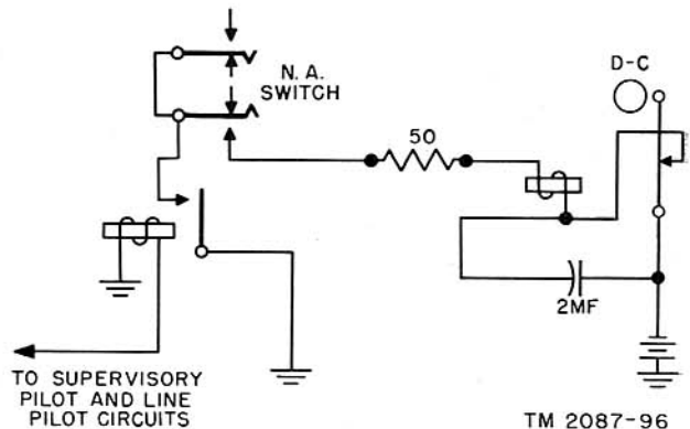
Figure 88. Night alarm circuit, schematic.
