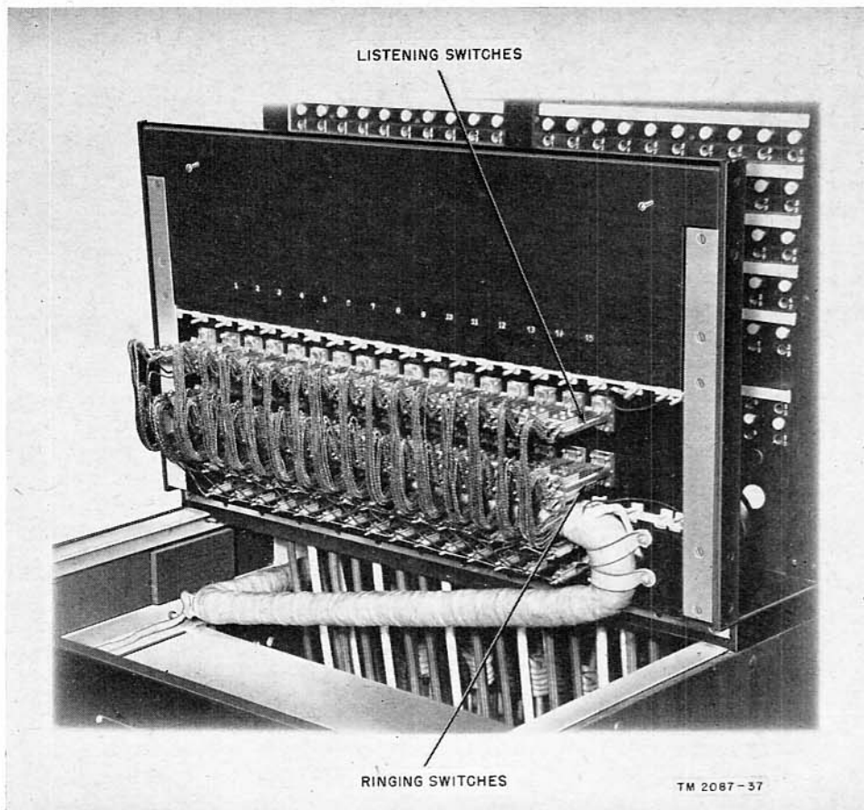
Figure 33. Switch shelf open, showing switches
