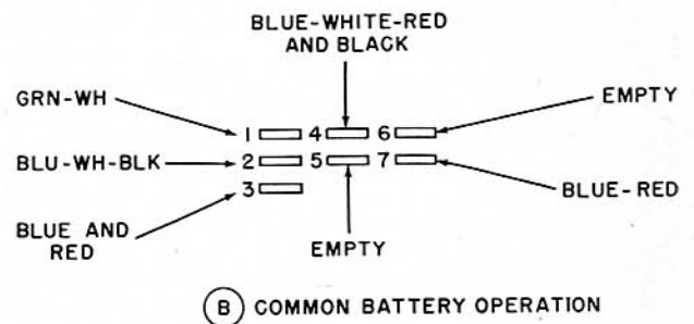
Figure 10. Kellogg line relay connection diagrams, spring relay numbering of 561-A line relay as viewed from terminal end.
