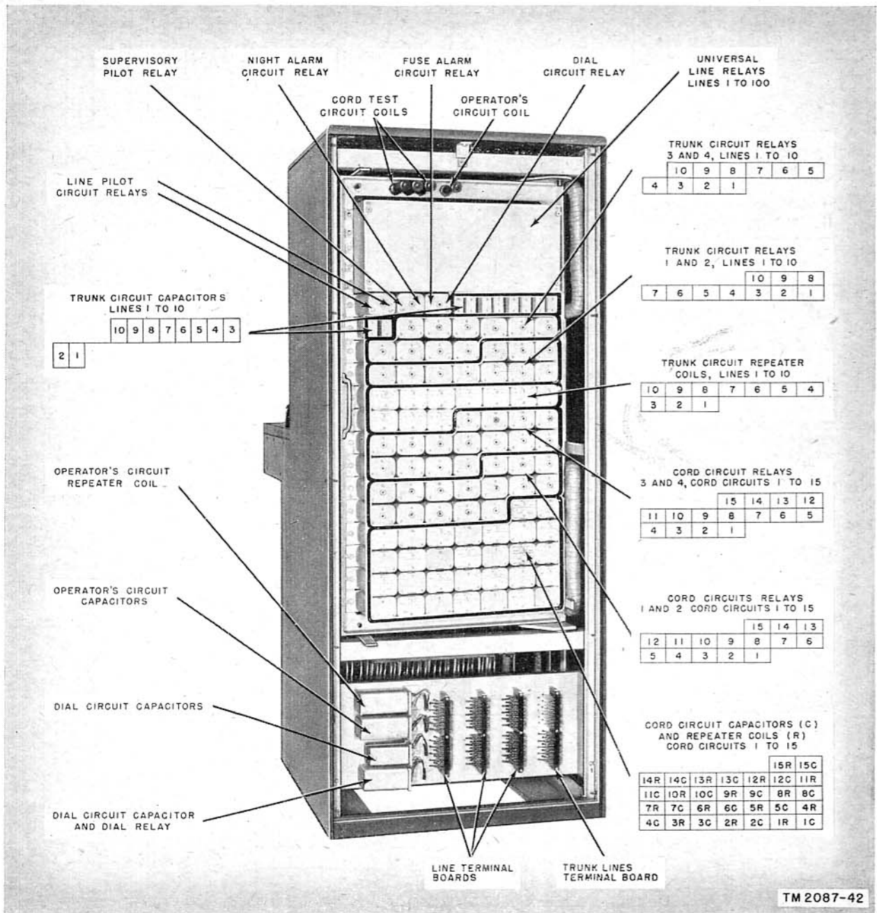
Figure 3. Switchboard SB-53( )/FTC (Kellogg type), rear view.
