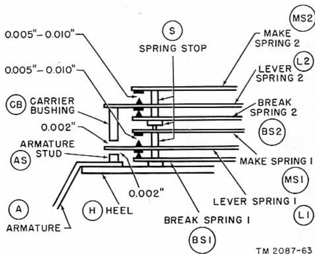
Figure 55. Multiple spring pile-up, normal position.
