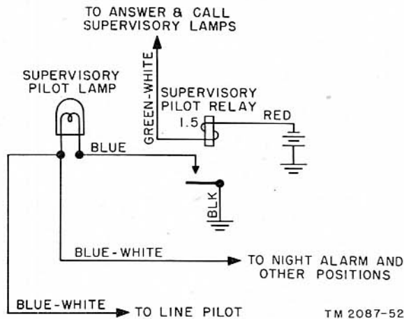
Figure 44. Supervisory pilot circuit, wiring diagram.
