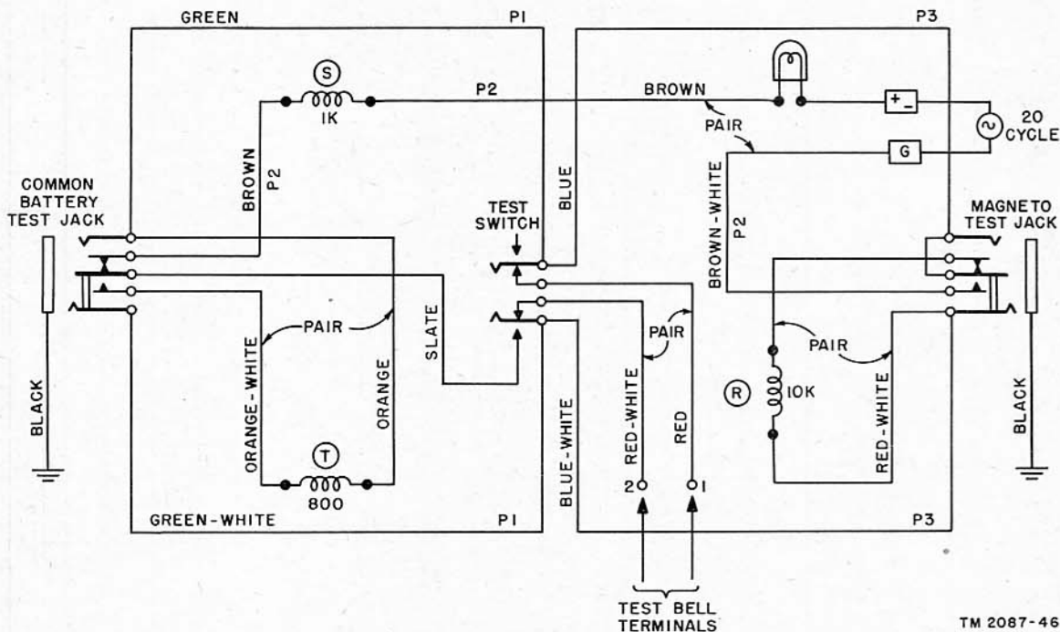
Figure 38. Cord test circuit, wiring diagram.
