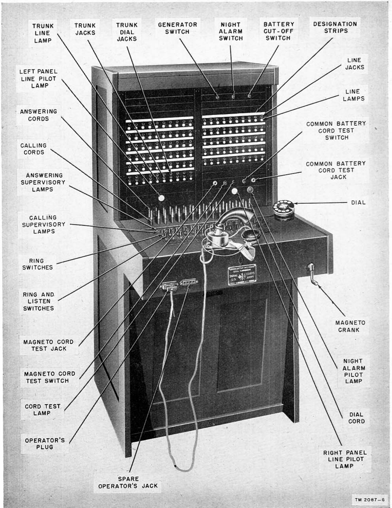
Figure 68. Switchboard SB-53( )/FTC (Stromberg-Carlson universal type 106), front view.
