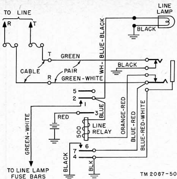
Figure 42. Universal line circuit connected for magneto operation, wiring diagram.
