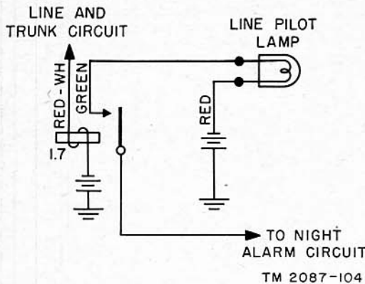
Figure 96. Line pilot circuit, wiring diagram.
