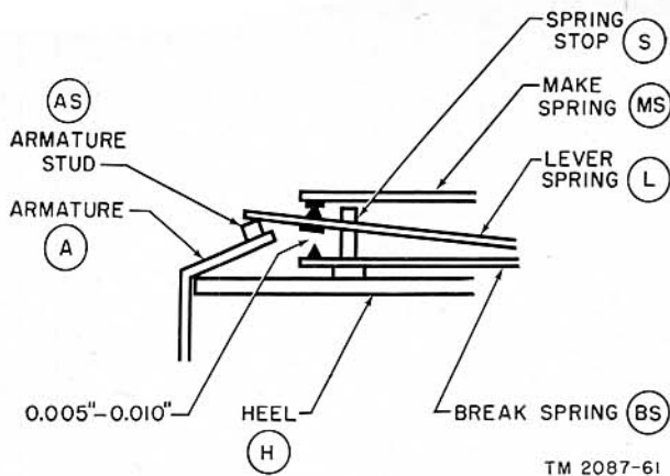
Figure 53. Break contact, operated position.
