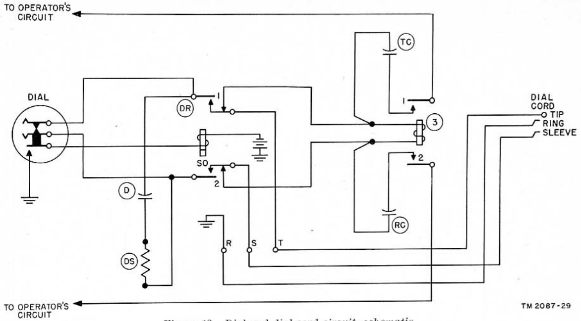
Figure 18. Dial and dial cord circuit, schematic.
