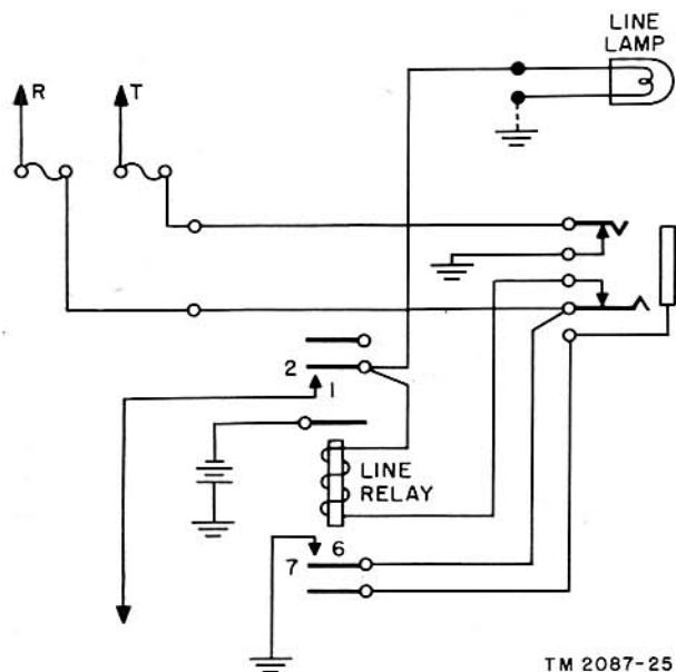
Figure 14. Universal line circuit connected for magneto operation, schematic.
