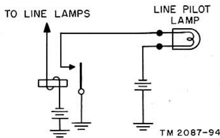
Figure 86. Line pilot circuit, schematic.
