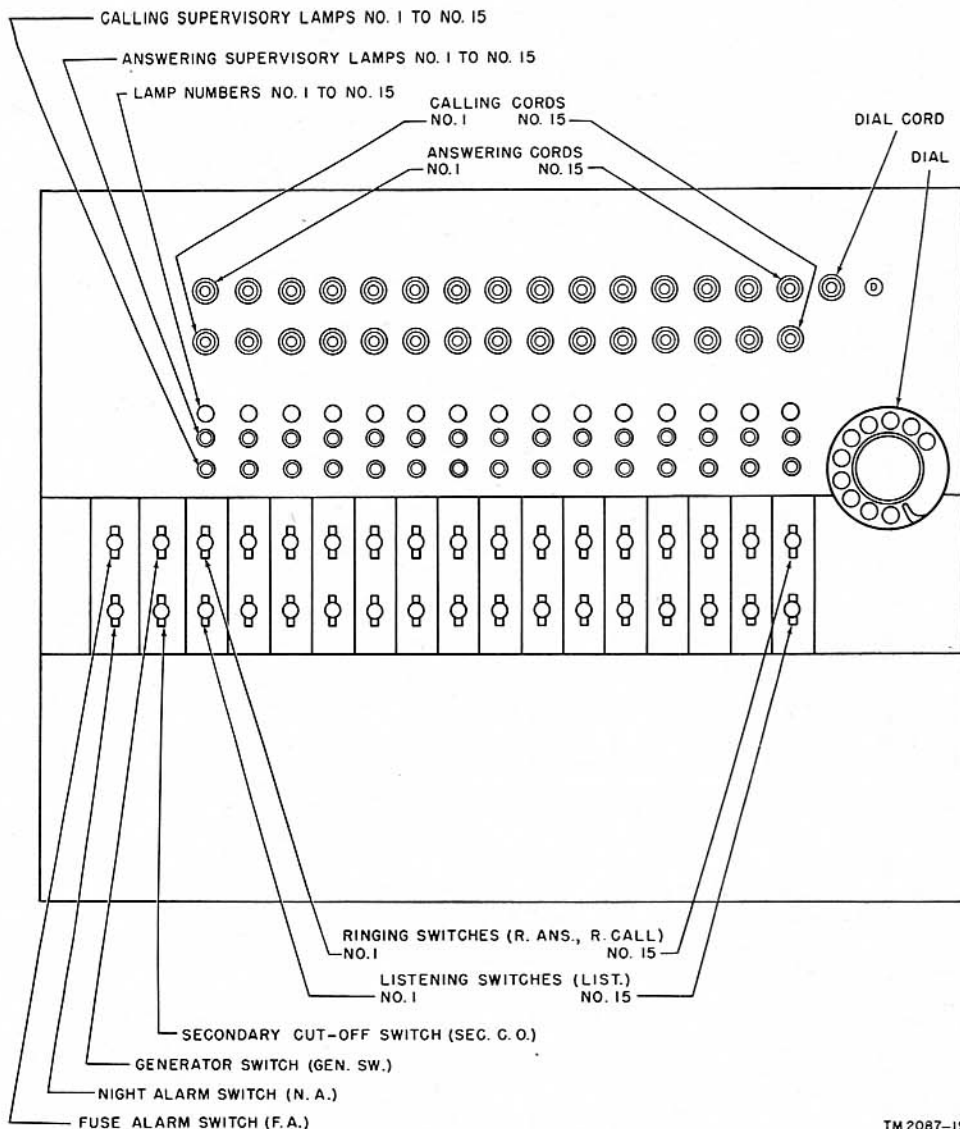
Figure 11. Switchboard SB-53( )/FTC (Kellogg type) switch shelf, top view, showing arrangement of cords, lamps, and switches.
