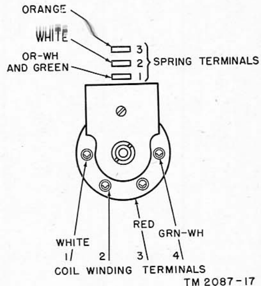
Figure 73. Switchboard SB-53( )/FTC (Stromberg-Carlson universal type 106), long lines relay wiring diagram.
