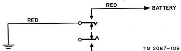
Figure 101. Battery switch circuit, wiring diagram.
