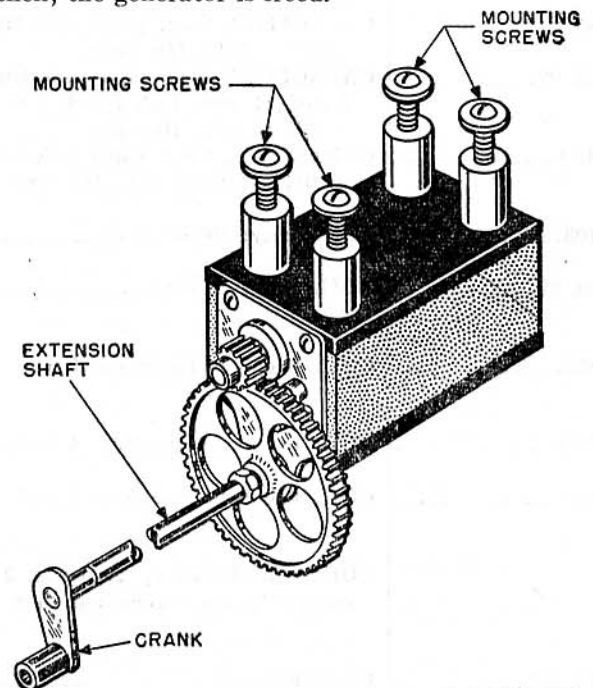
Figure 112 (Added) Hand generator supplied with Switchboard SB-53A/FTC, overall view.
