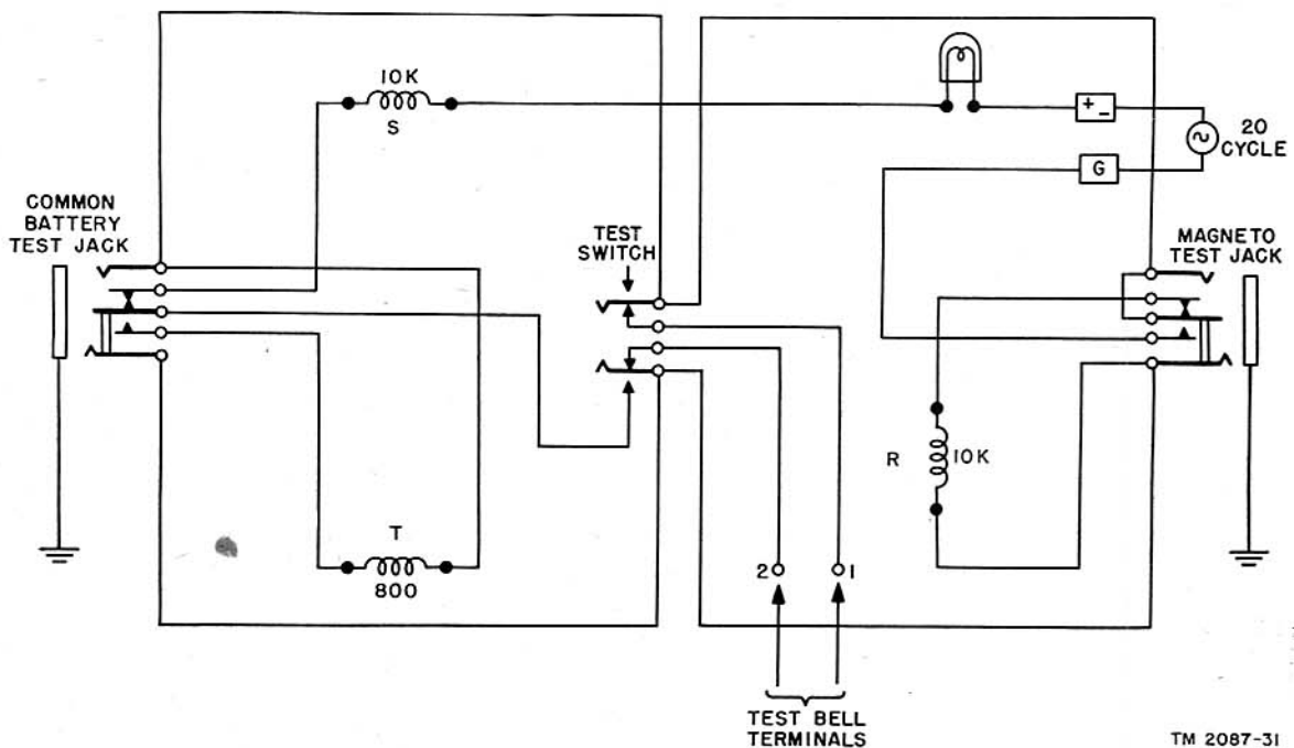
Figure 20. Cord test circuit, schematic.
