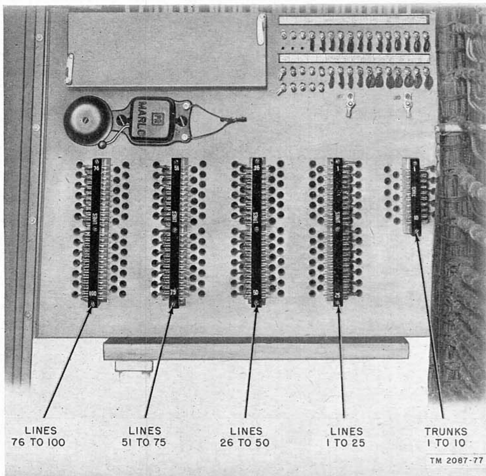
Figure 71. Fanning and terminal boards.
