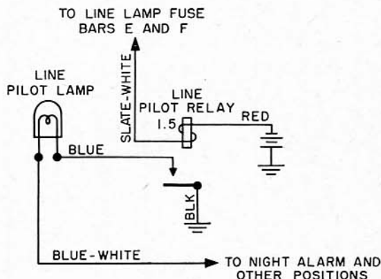
Figure 43. Line pilot circuit.
