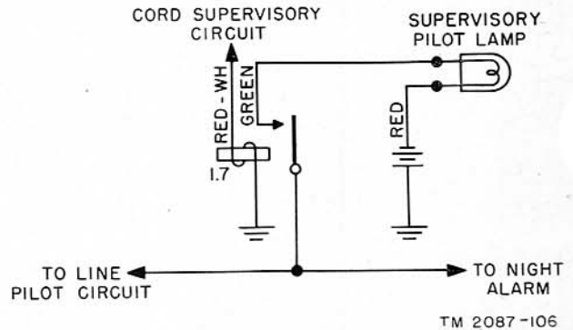
Figure 98. Supervisory pilot circuit, wiring diagram.
