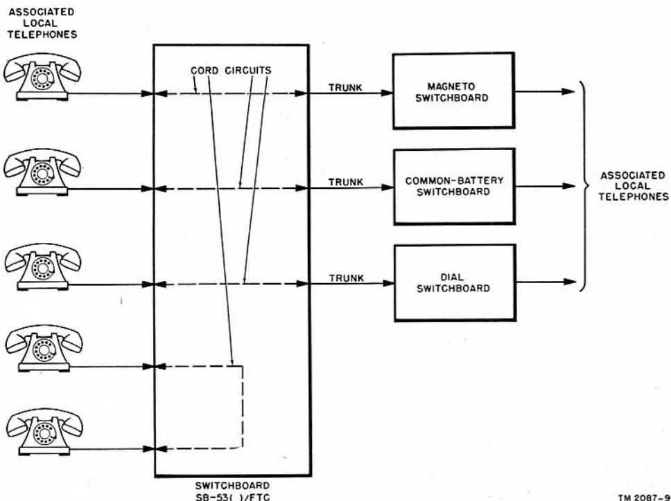
Figure 5. Switchboard SB-53( )/FTC, possible connections, block diagram.
