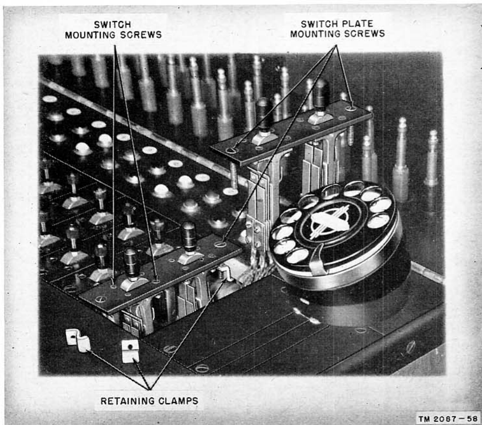
Figure 50. Switch plate mounting screws and retaining clamps.
