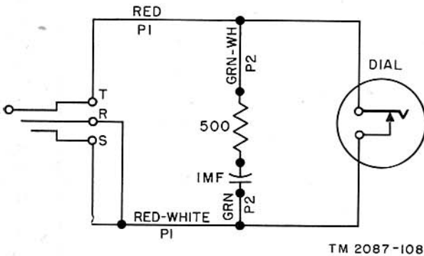
Figure 100. Dial and dial cord circuit, wiring diagram.
